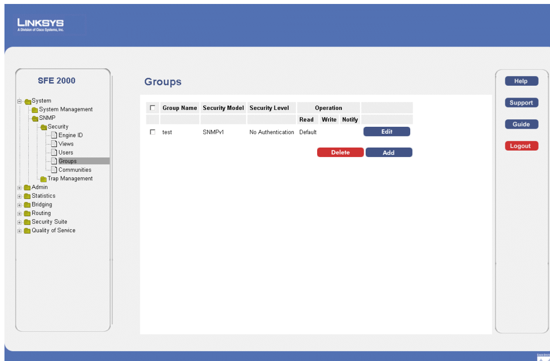
SNMP Groups Profile Page
